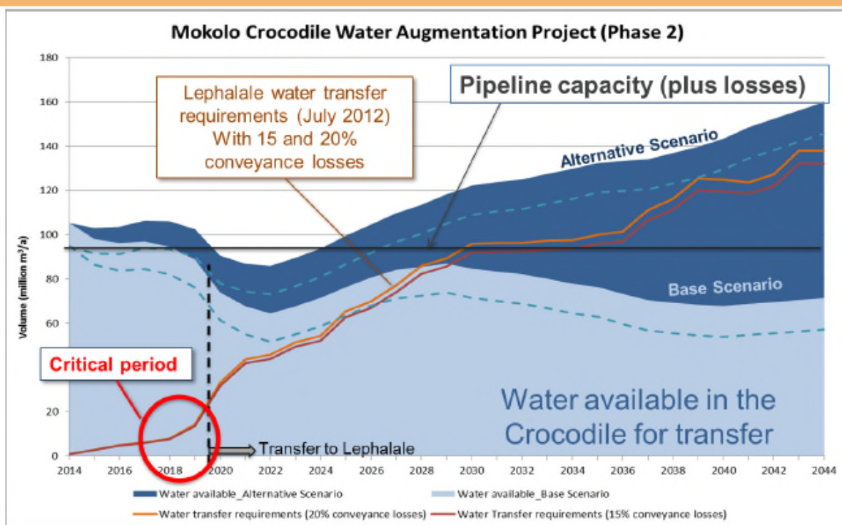
Surplus water available from Crocodile West River System for augmentation to the Mokolo 94
