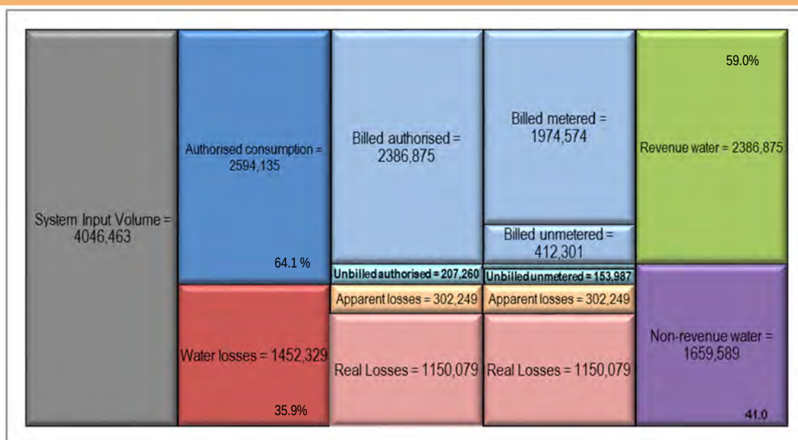
Figure 3-8: National IWA Water Balance for Water Losses and Non-Revenue Water Mm³/a
